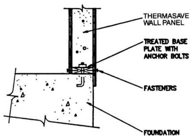
WALL BASE DETAIL
