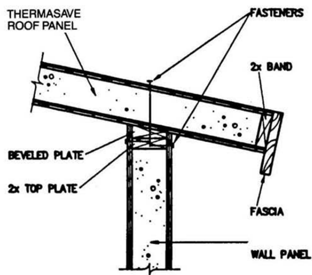
PITCHED ROOF AT WALL
